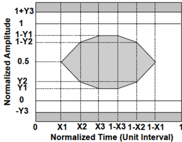
Figure. Eye Mask Definition
