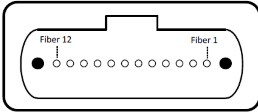
Outside view of the QSFP module MPO
